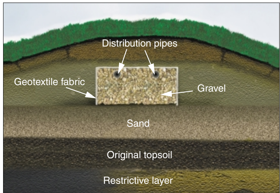
Figure 2: A mound system is placed above the natural surface of the ground.
